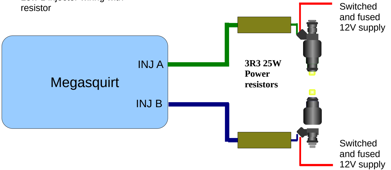
Diagram showing two channels with one injector per channel and 3.3 ohm series resistors. Repeat for Inj C-H as required.
