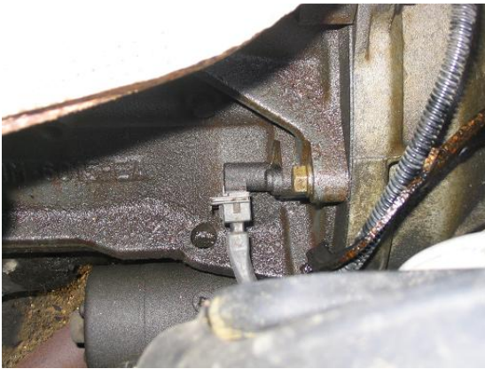
Escort / Fiesta location on engine flange above starter.
