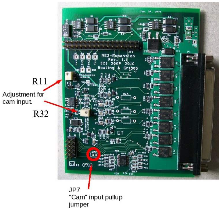
MS3X card cam configuration.
