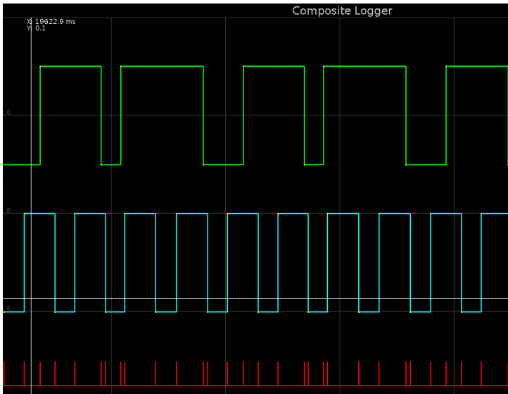
Composite log of 4G63 CAS (from Miata) recorded using "Log crank & Cam" mode.
