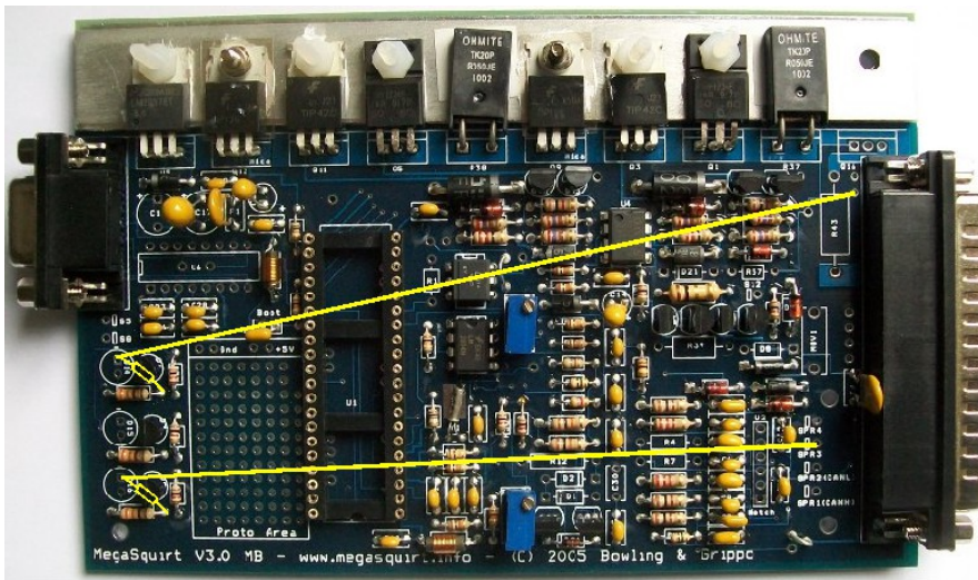
Add two 1k 1/8W resistors as shown. One on D14, one on D16
