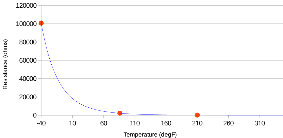
Temperature sensor resistance
