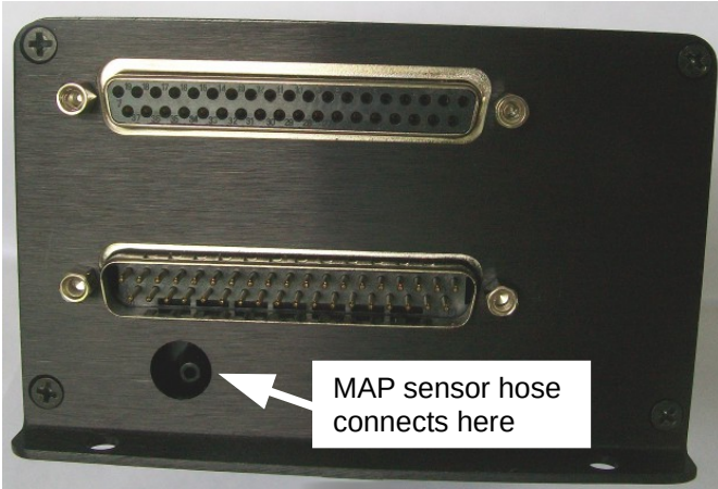
(MAP sensor is centred on MS3X/V3.57)
